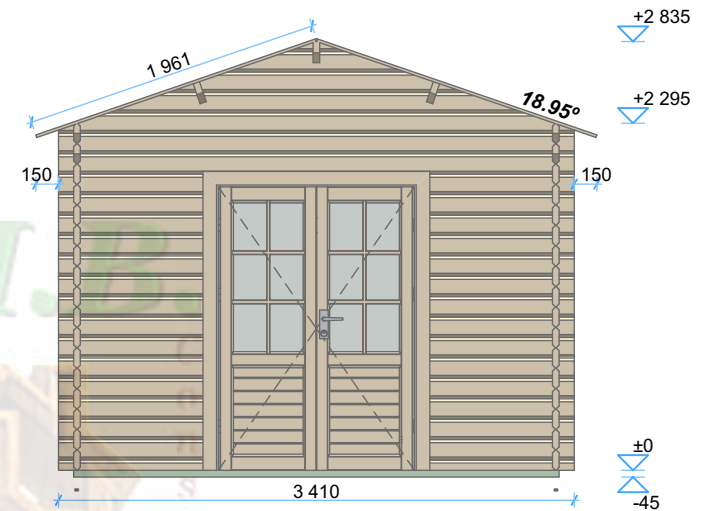
North Elevation
