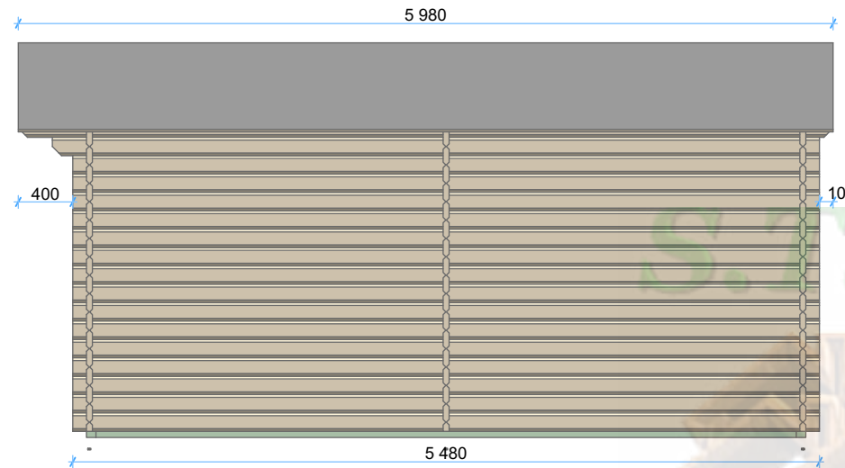
West Elevation
