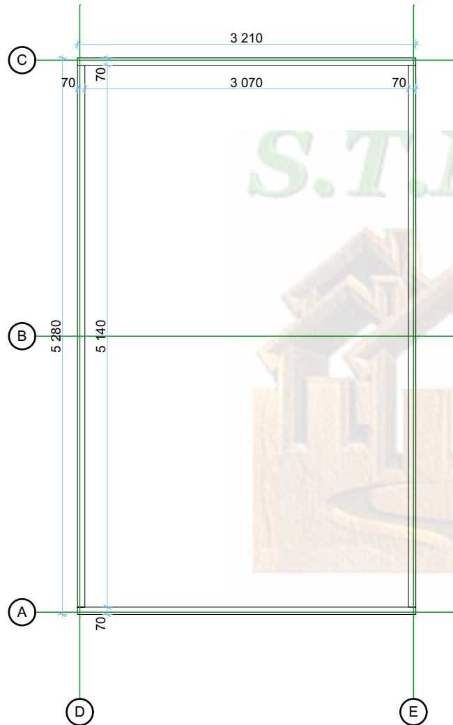
Floor bearers
